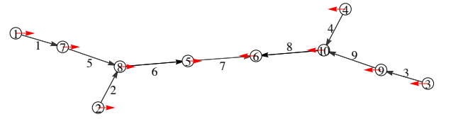
Fig. 5: The gray lines joining the buses show the magnitude of the power flow with the grayscale and the direction of the power flow with the arrows. Each line is numbered as shown. The red arrows at each bus show the oscillation mode shape; that is, the magnitude and direction of the entries of the right eigenvector x_\delta associated with the complex eigenvalue \lambda_{3i} . 1, 2, 3 and 4 are generator buses and 5 and 6 are load buses.
