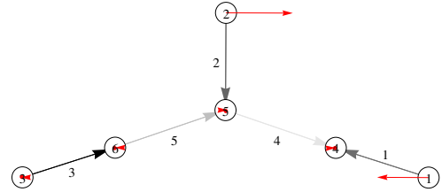
Fig. 8: Six-bus system: The gray lines joining the buses show the magnitude of the power flow with the grayscale and the direction of the power flow with the arrows. Each line is numbered as shown. The red arrows at each bus show the oscillation mode shape; that is, the magnitude and direction of the complex entries of the right eigenvector x_\delta associated to the critical complex eigenvalue \lambda_{2i} . Buses 1 and 2 are antinodes and buses 3,4,5,6 are nodes.
