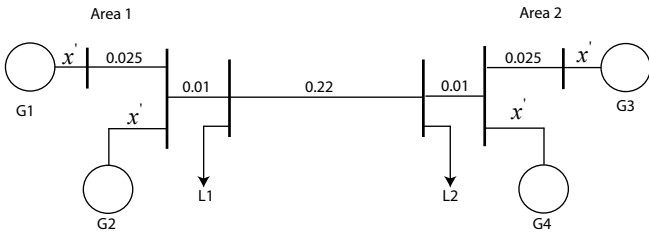
Fig. 4: 10-bus system
