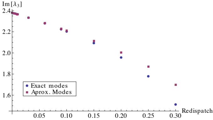
Fig. 7: Exact and approximate mode frequencies versus amount of redispatch in the 10-bus system.
