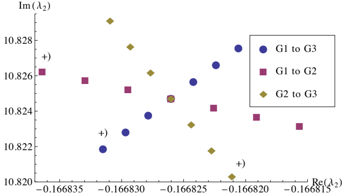
Fig. 9: Eigenvalues for redispatches of the 6-bus system.
